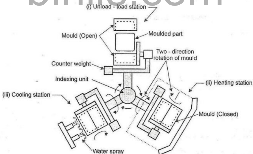
Figure 5.13 Rotational Moulding
