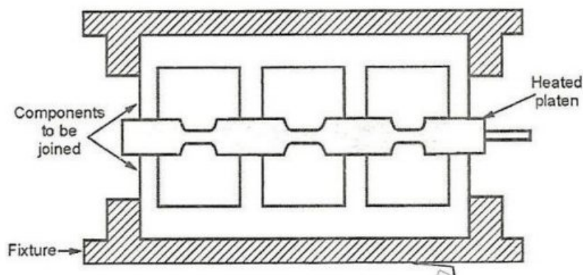
Figure 5.16 Hot-platen welding
