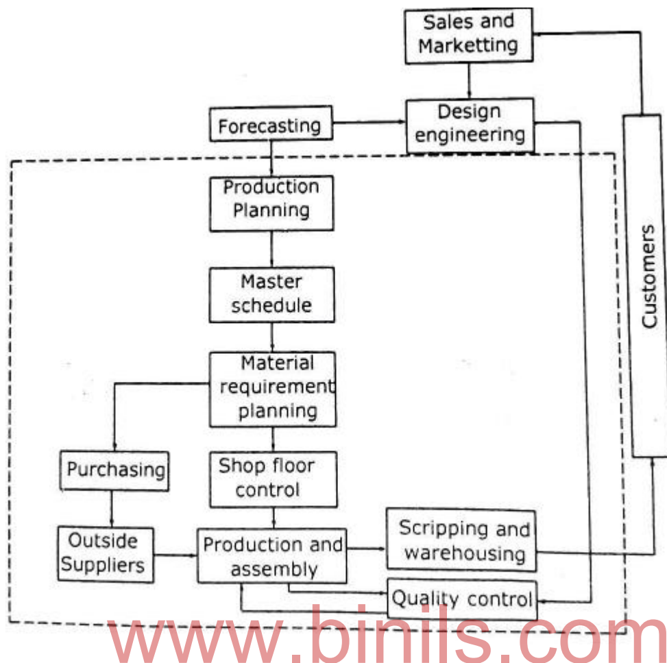
Figure 2.10 Computer integrated production management system
