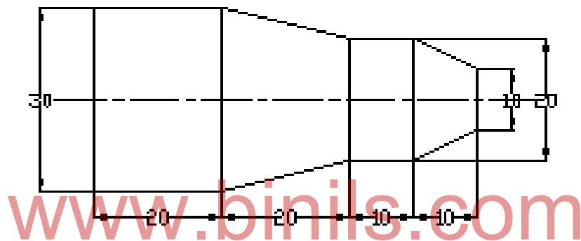
Figure 3.7 Linear interpolation
