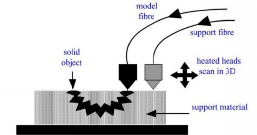
Figure 3.16 Schematic of the FDM process
