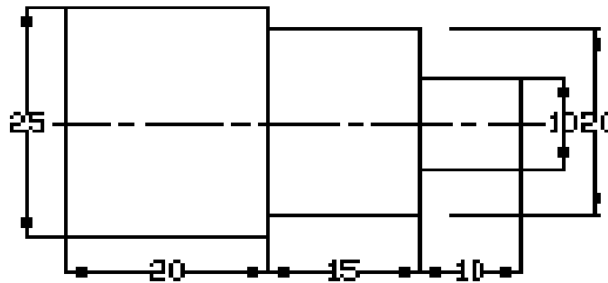
Figure 3.9 Box turning
