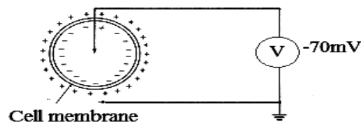
Fig 1.2 Resting potential
