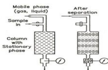
Fig.1.26 (a) Chromatography
