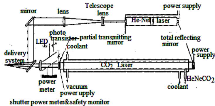
Fig.5.4 Block diagram of CO 2 Laser
