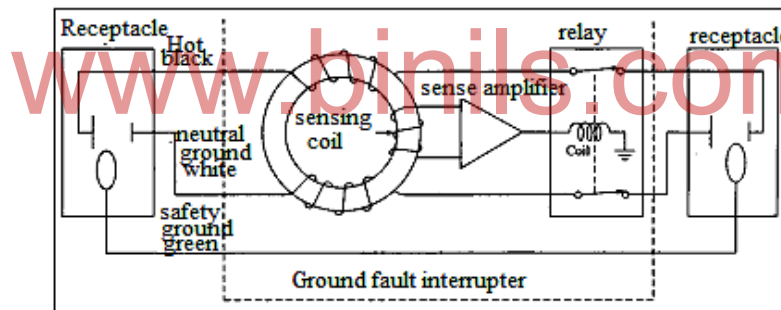
Fig. 4.13 Ground Fault Interrupter ( GFI )
