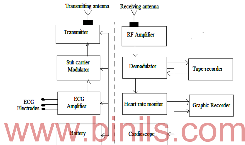
Fig.4.3 Block diagram of a single channel telemetry system
