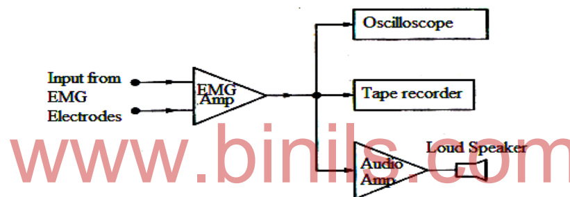
Fig.2.23 Block diagram of EMG Recorder
