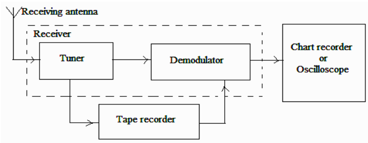
Fig.4.2 (b) AM or FM Receiver in Biotelemetry system
