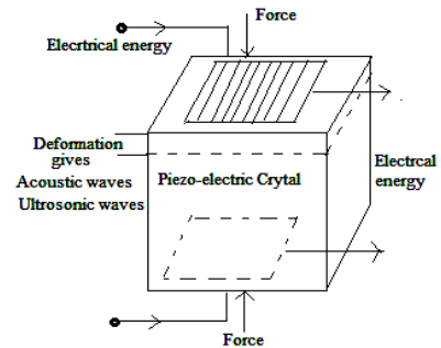
Fig.5.6 Generation of Ultrasonic waves
