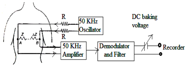
Fig.1.22 Measurement of Respiration rate (Impedance Pneumography)
