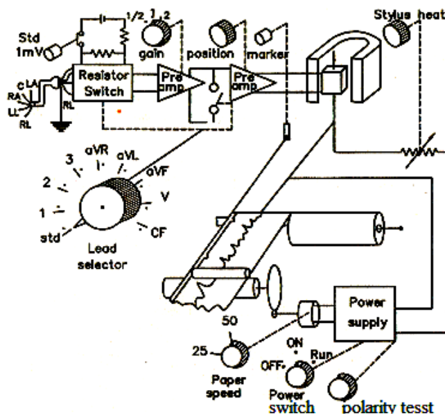
Fig.2.12 ECG Recorder
