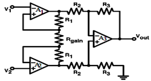
Fig.2.11 Instrumentation Amplifier
