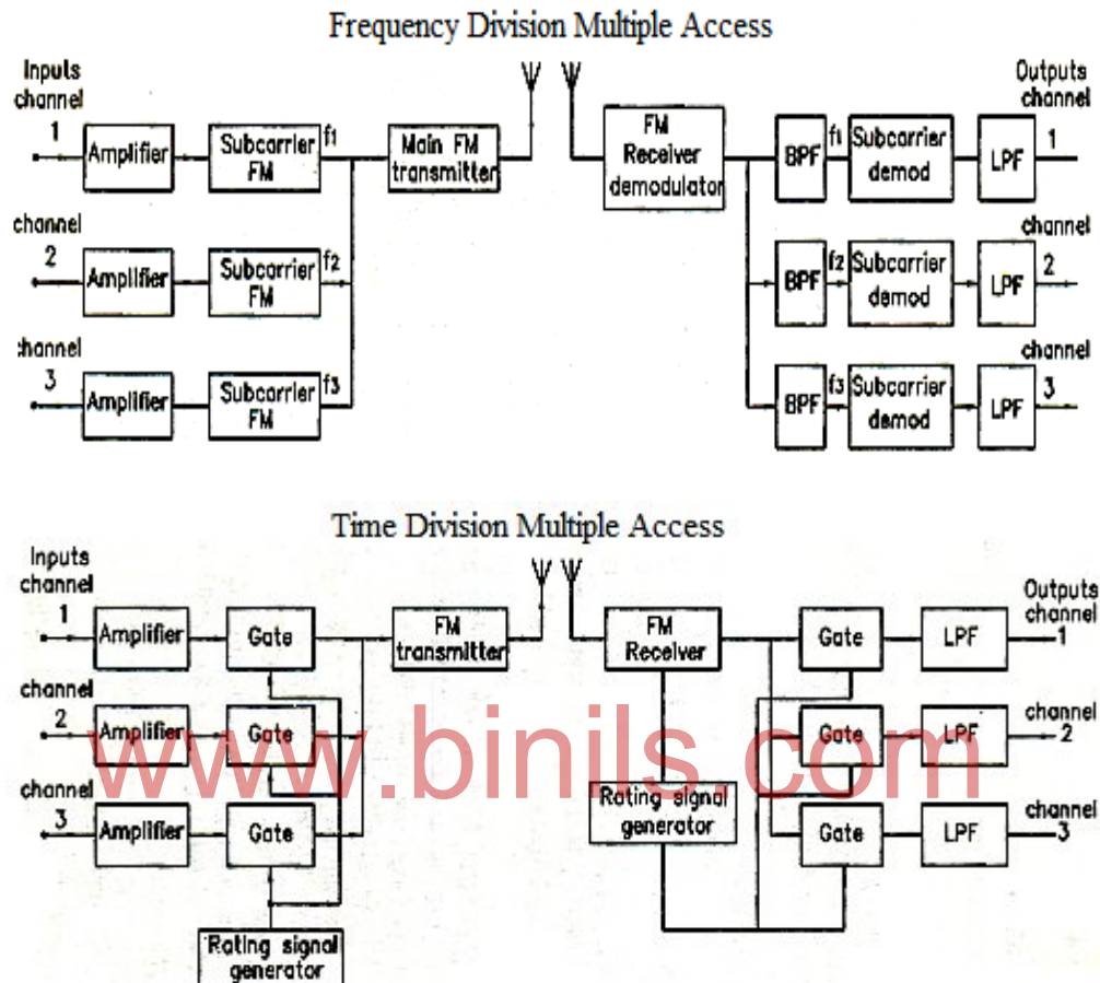
Fig.4.4 Multi channel telemetry system
