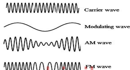
Fig.4.2 (c) AM and FM Wave
