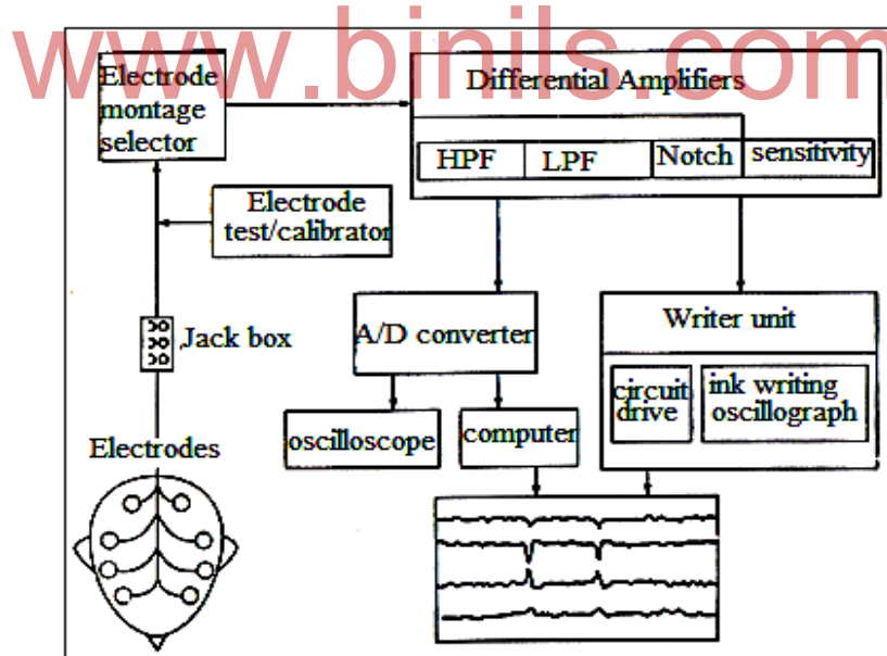
Fig 2.16 EEG Recording machine
