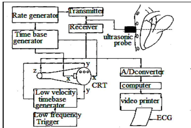
Fig.5.8 Block diagram of Echocardiography
