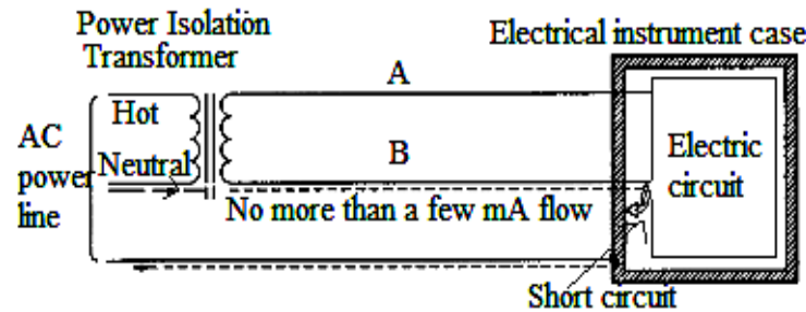
Fig.4.16 Prevention of shock hazard in Electro surgical units
