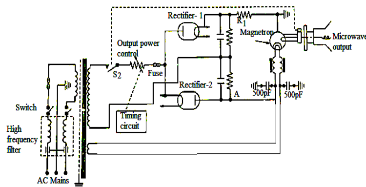
Fig.3.14 Circuit diagram of Microwave diathermy machine
