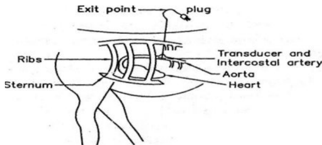
Fig. 1.6 Implantation technique of pressure measurement
