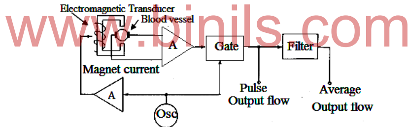
Fig.1.19 Magnetic Blood Flow Meter
