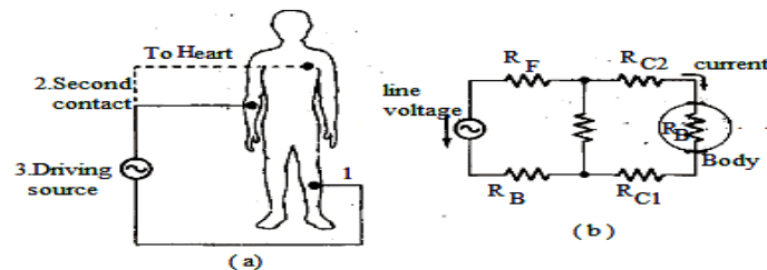
Fig.4.11 Grounding
