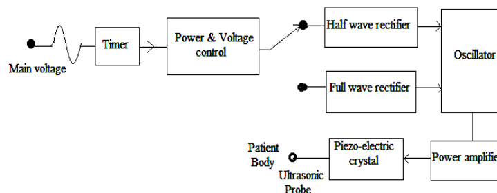
Flig.3.15 Block diagram/Circuit diagram of Ultrasonic Diathermy unit
