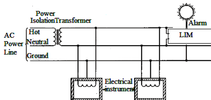
Fig.4.17 Prevention of shock hazard due to burns and explosion
