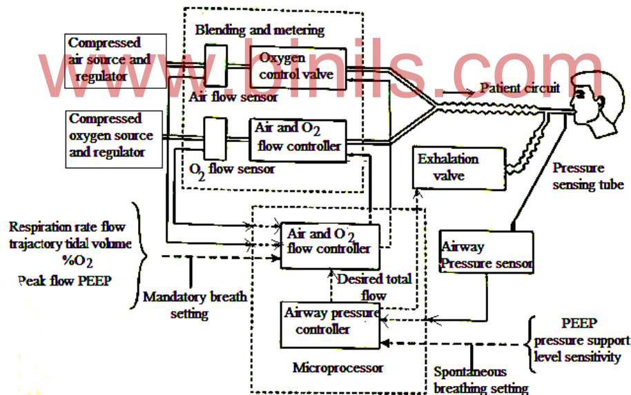
Fig.3.17 Block diagram of Modern ventilator
