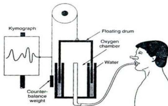
Fig.1.23 Basic water sealed Spiro meter (Measurement of Lung Volume)
