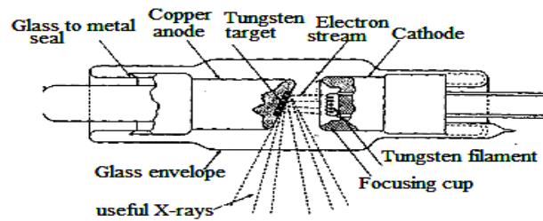
Fig.5.10 Generation of X-rays
