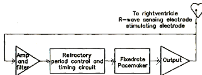
Fig.3.3 R-wave triggered demand pacemaker.
