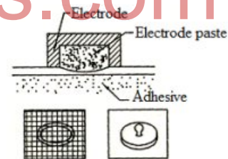
Fig.2.9 Adhesive type Surface electrode
