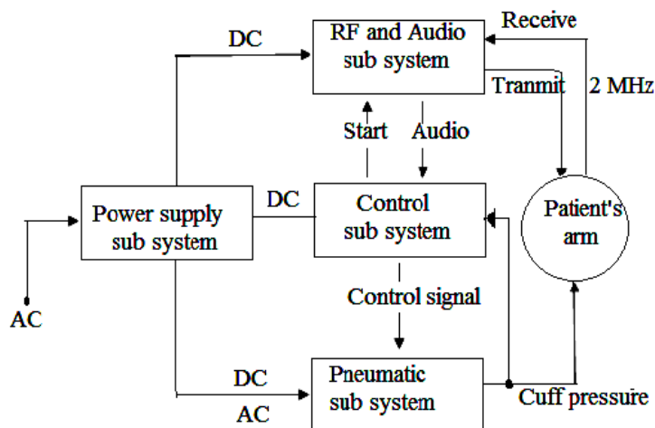
Fig.1.17 Ultrasonic BP measurement(Indirect method of blood pressure measurement)
