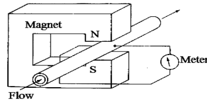
Fig.1.18 Principle of Electromagnetic Blood flow meter
