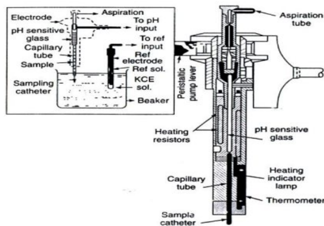
Fig.1.21 Measurement of Blood pH(pH electrode)
