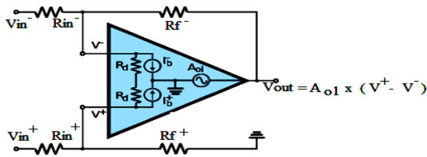
Fig.2.10 Differential Amplifier
