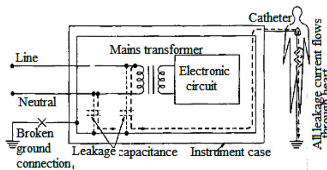
Fig.4.8 Situation of Micro Shock hazard
