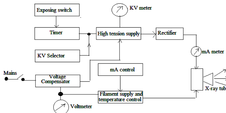
Fig.5.11 Block diagram of X-Ray Apparatus
