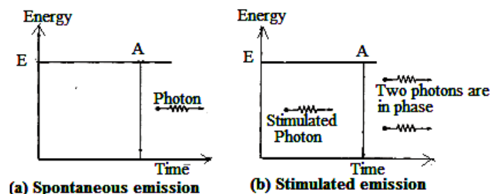
Fig.5.1 Laser principles
