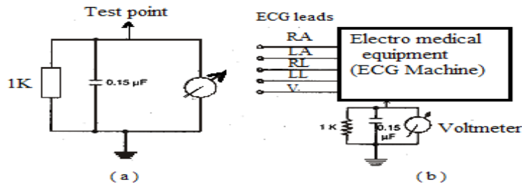
Fig.4.10 Leakage current measurement
