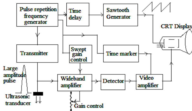
Fig.5.7 Block diagram of Pulse-echo signal(Ultrasonic imaging )
