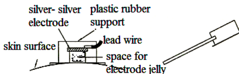
Fig.1.11 Floating type surface electrode
